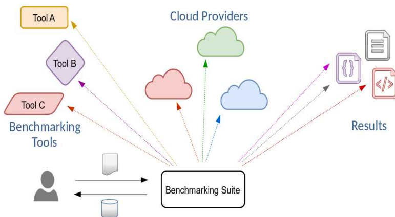
Illustration 1: The Benchmarking Suite is a single access point to Cloud benchmarking that automates and simplifies the execution of tests and the analysis of results.
